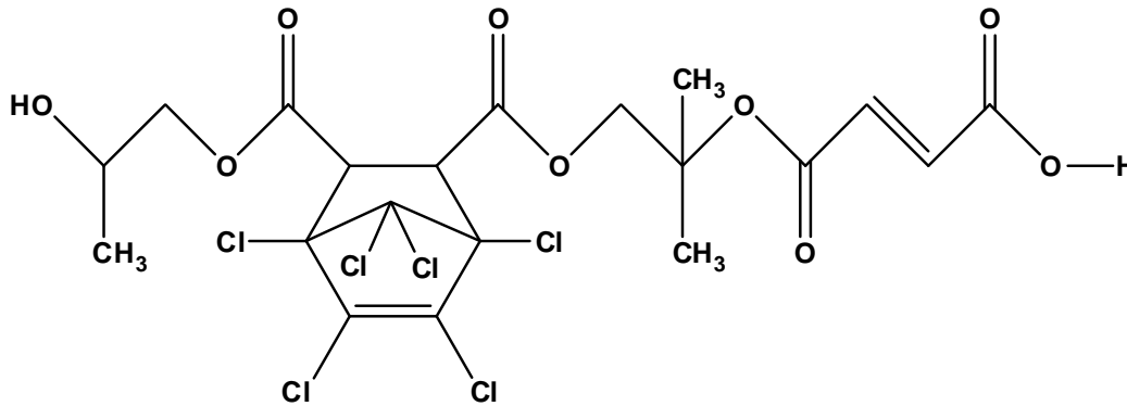
Figure 3. Chlorendic Polyester Resin Polymer Structure
